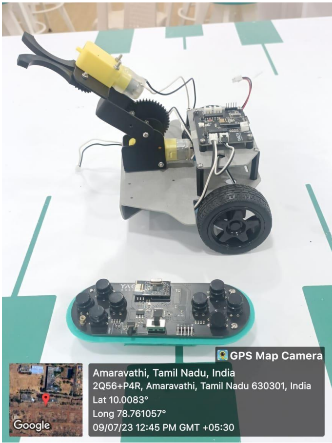
Pick & Place Robot
